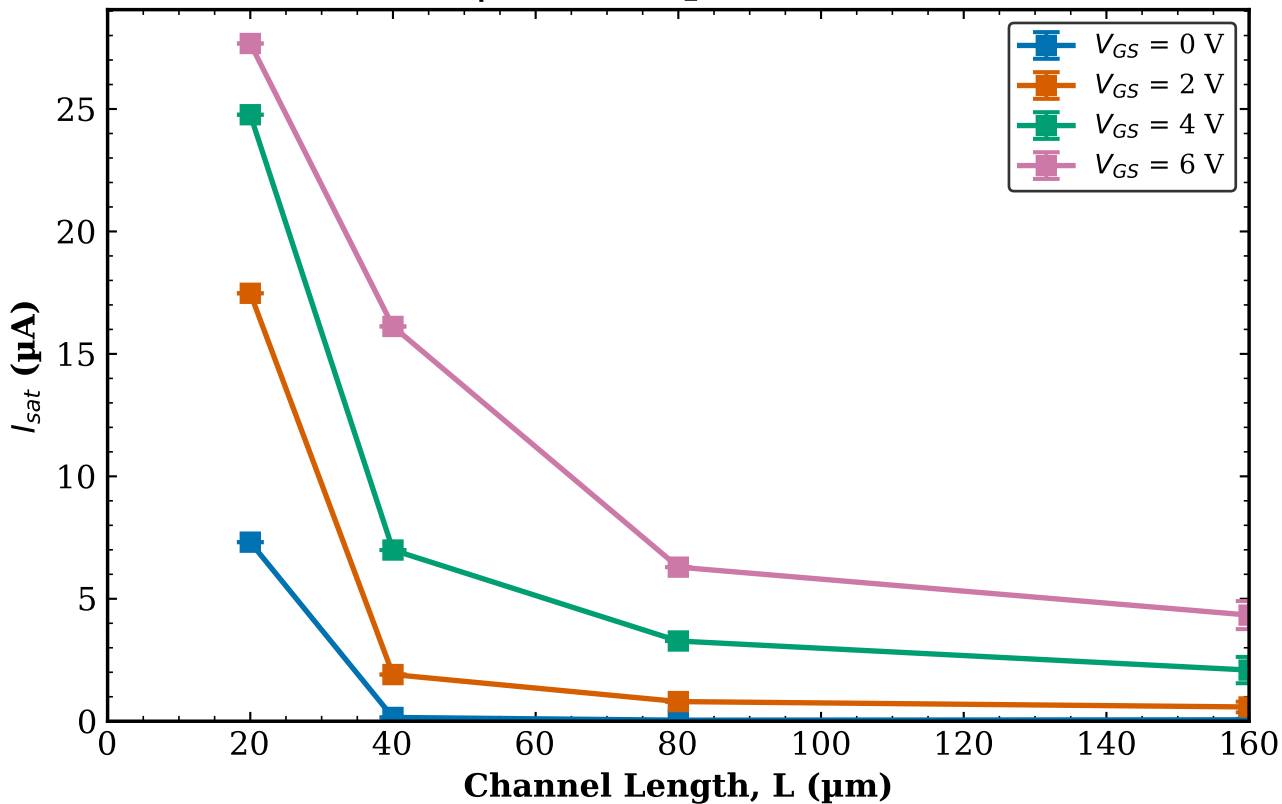
TFT2 Combined (Tr. 1 & 2) I_{sat} vs L | W = 50 \mu\text{m} (mean \pm std)
